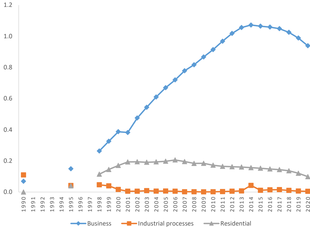
Chart B11. F-gas Emissions by National Communications Category, 1990 to 2020. Values in MtCO 2e
