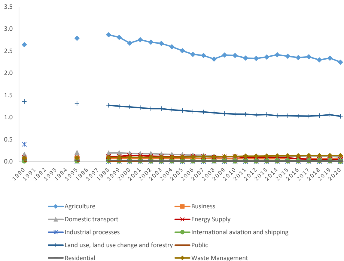
Chart B10. Nitrous Oxide (N 2 O) Emissions by National Communications Category, 1990 to 2020. Values in MtCO 2e
