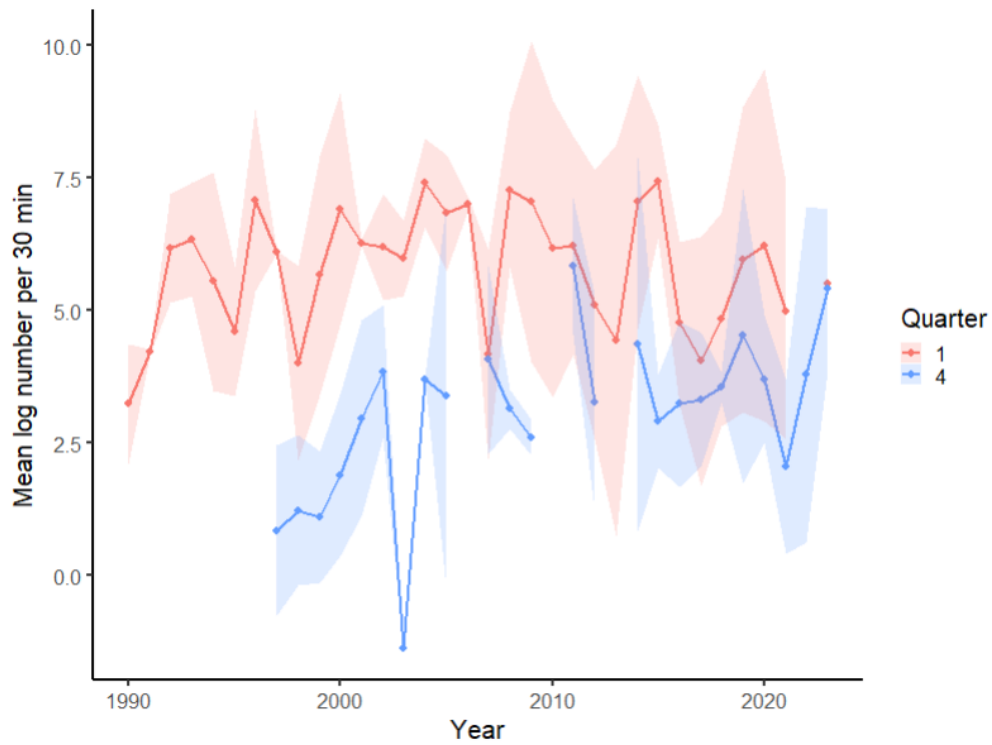
Figure 12 (from consultation document ). Mean log number per standard tow of herring in the Clyde from bottom trawl surveys in Q1 and Q4. Note that this is based on low sample sizes (2 – 4 hauls per year in the Clyde) and bootstrapping has been used to calculate confidence intervals. Gaps refer to years where no survey took place.
